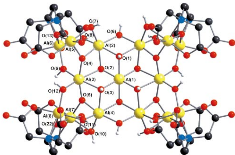
Figure 1. The supramolecular structure of the cluster ion [\text{Al}_{15}(\mu_3\text{-O})_4(\mu_3\text{-OH})_6(\mu\text{-OH})_{14}(\text{hpdt}\text{a})_4]^{3-} in 1a . The hydrogen atoms on the peripheral ligands are omitted for clarity. Al–O bond lengths (Al–O–Al angles) are in the ranges: 1.847(3)–2.083(3) Å (92.3(1)–101.7(2)°) for Al–( \mu_3 -OH); 1.824(3)–1.969(4) Å (92.5(1)–130.0(2)°) for Al–( \mu_2 -OH); 1.753(3)–1.841(3) Å (101.8(2)–142.8(2)°) for Al–( \mu_3 -O). The Al–N bond lengths are in the range 2.036(4)–2.116(4) Å.
